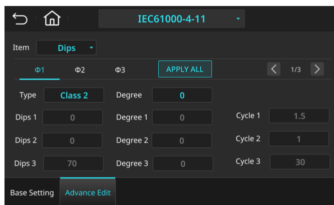
Figure 10: IEC61000-4-11 Dips Setting
