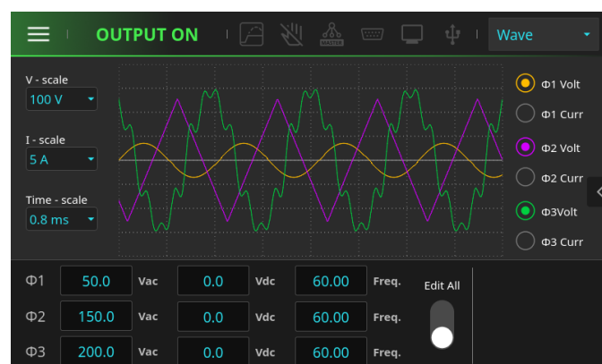
Figure 5: Waveform Monitoring Function
