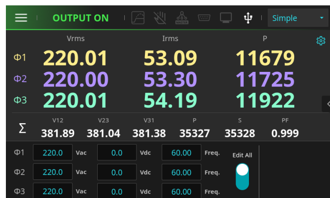
Figure 4: Real Time Measurement Display
