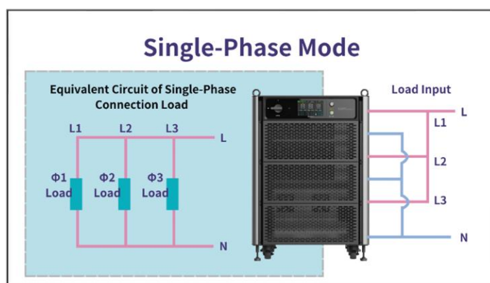
Figure 5: Single-Phase Mode
