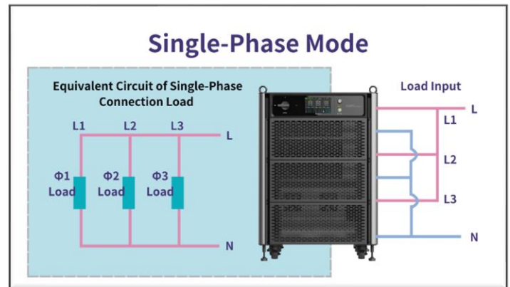
Figure 5: Single-Phase Mode
