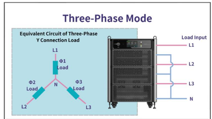
Figure 6: Three-Phase Mode
